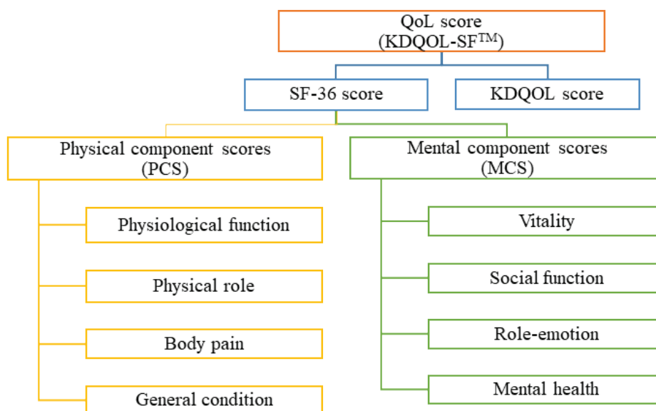
Figure 1. Scores of the items in the KDQOL-SF questionnaire to assess QoL
